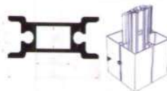
HB-322 60方柱连接件 Connecting Lock/60mm
