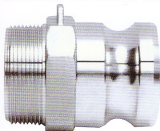
不锈钢快速接头 TYPE-F STAINLESS STEEL CAMLOCK COUPLINGS MALE ADAPTER x MALE THREAD
