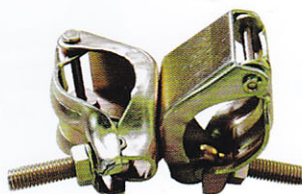
韩式冲压直角扣角 KOTEAN STYLE PRESSED DOUBLE COUPLER
