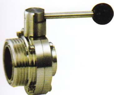
一端螺纹 / 一端焊接蝶阀 ONE END THREADED/ONE END WELDED BUTTERFLY VALVE
