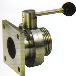
一端法兰 / 一端螺纹蝶阀 ONE END FLANGED/ONE END THREADED BUTTERFLY VALVE
