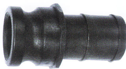
塑料 PP 快速接头 TYPE-E POLYPROPYLENE CAMLOCK COUPLINGS MALE ADAPTER x HOSE SHANK
