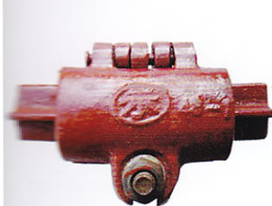
对接扣件 BUTT-JOINED FASTENING PIECES
