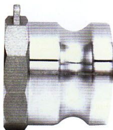
不锈钢快速接头 TYPE-A STAINLESS STEEL CAMLOCK COUPLINGS MALE ADAPTER x FEMALE THREAD
