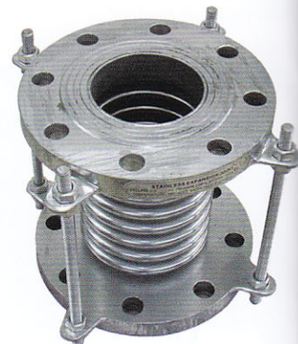
轴向型补偿器 AXIAL DIRECTION COMPENSATOR
